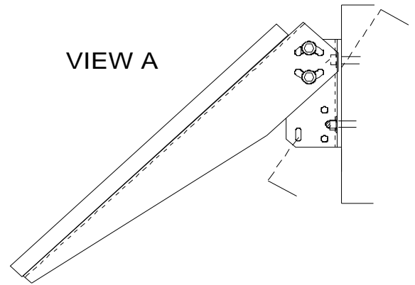
Mounting On Vertical Or Steeply Sloping Flat Surface Using (2) Lag Screws Or Bolts.
