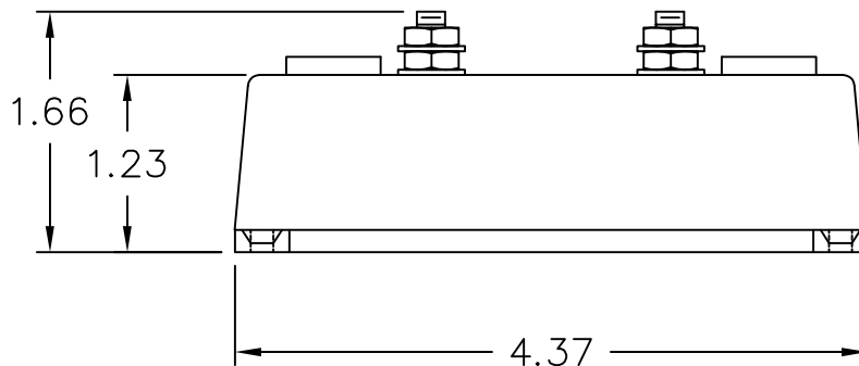
SIDE VIEW
