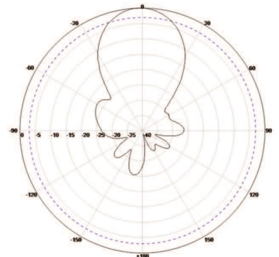
E Plane
