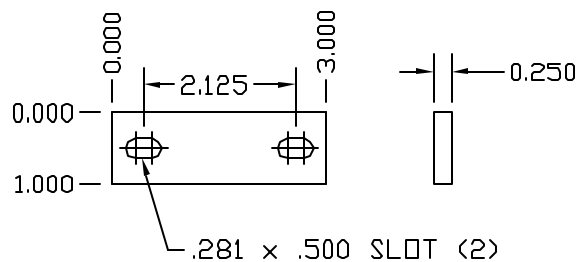
SPLICE PLATE
