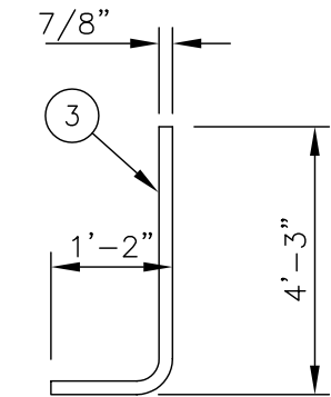
REBAR DETAIL
