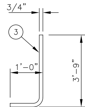
REBAR DETAIL (PIER VERTICAL REBAR)
