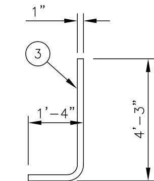
REBAR DETAIL (PIER VERTICAL REBAR)
