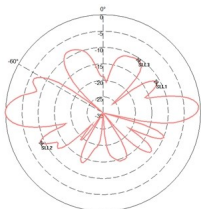
E-Plane Pattern
