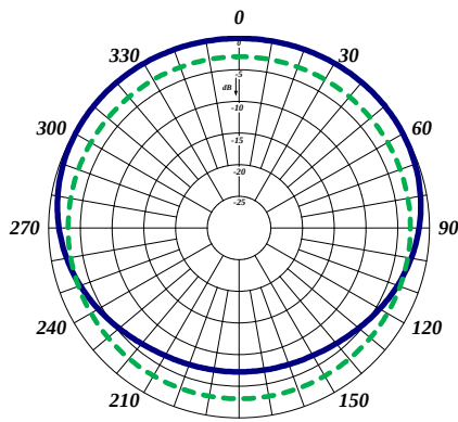
Quarter-wave Spacing Horizontal
