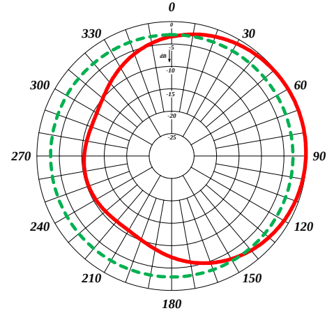
Vertical Pattern
