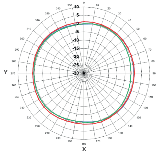
H Plane
