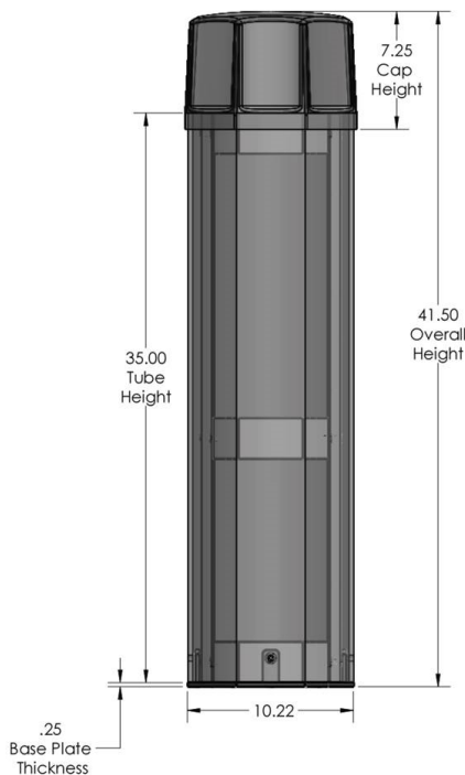
Octagonal Cap Bollard
